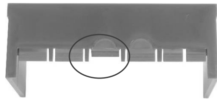
Tab pushed backwards to accommodate 1.5mm 2 cable
