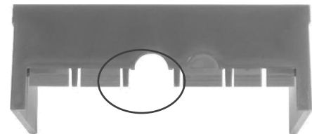
Circular knockout removed to accommodate 5-core modular wiring cable
